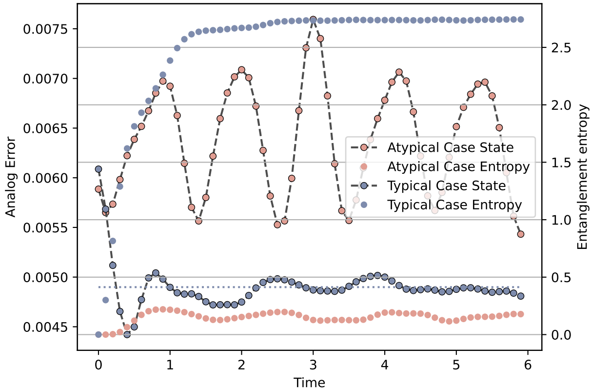
2D-lattice QIMF, one segment evolution with disorder
